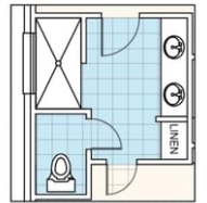
3'X6' DOORLESS SHOWER W/ ENCLOSED WATER CLOSET
